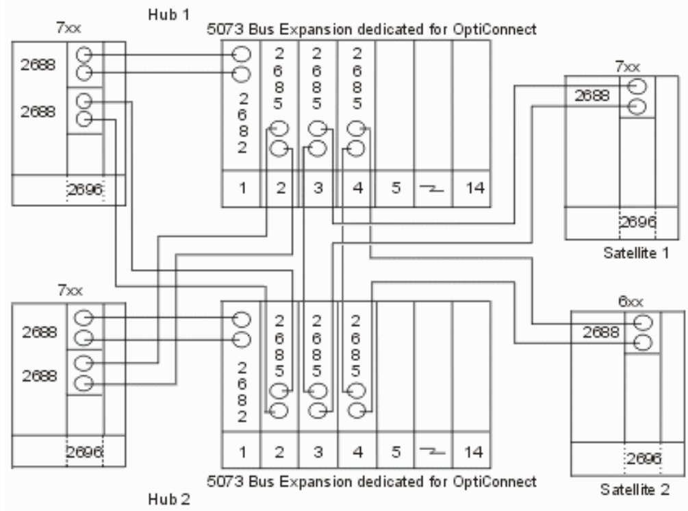
Figure 6. Dual-Hub SPD OptiConnect Cluster
