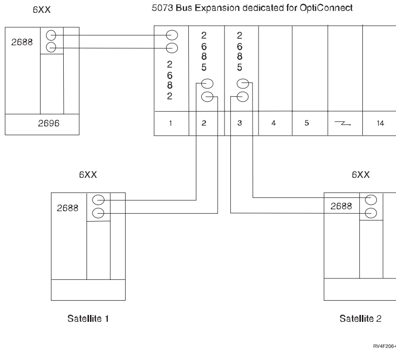
Figure 5. Single-Hub SPD OptiConnect Cluster
