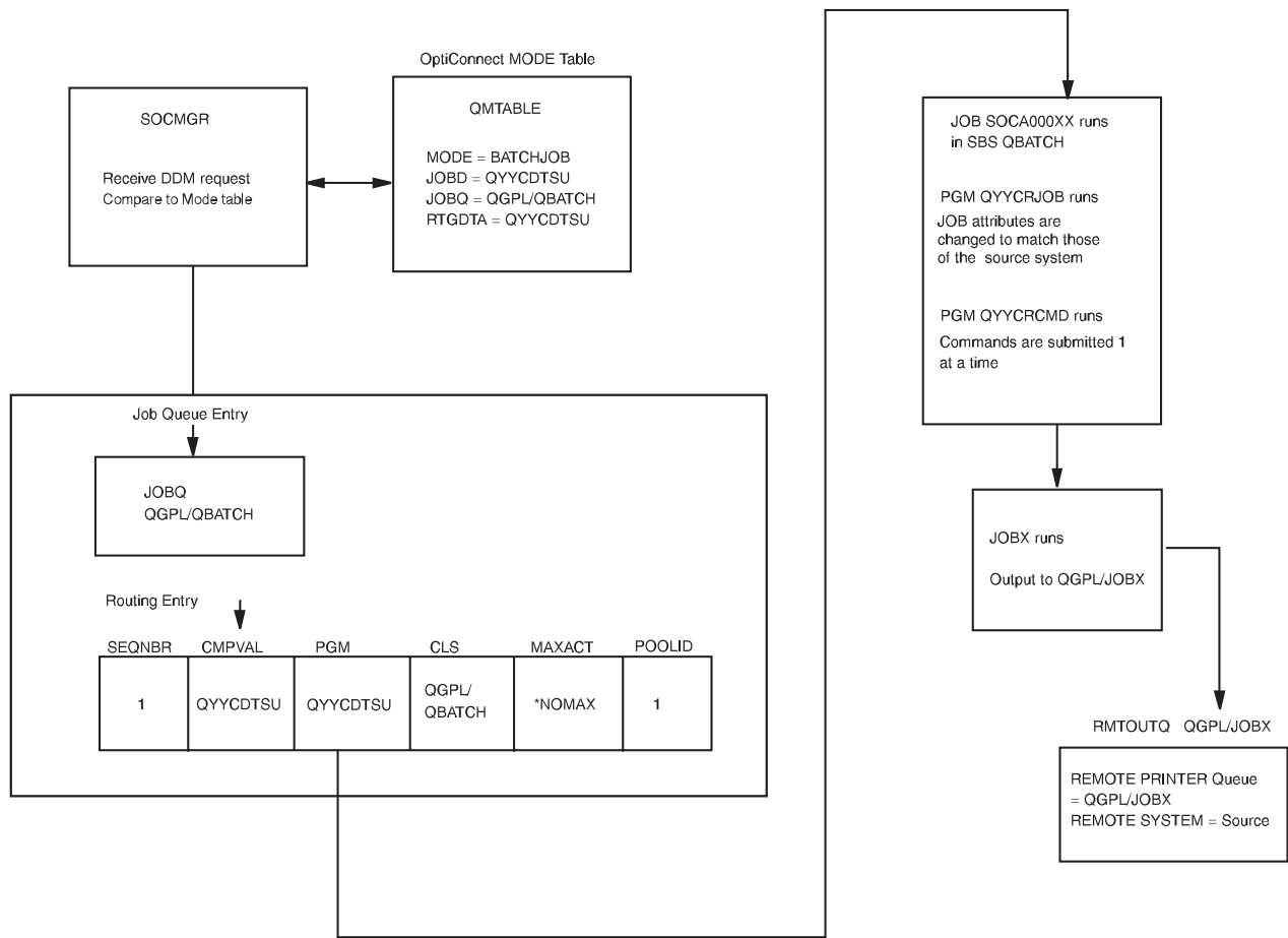
Figure 37. Remote Job Submission Target System
