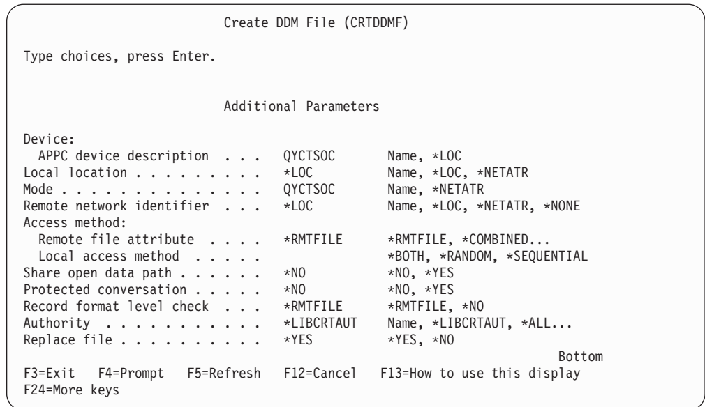
Figure 25. Creating a DDM file to use OptiConnect (View 2)
